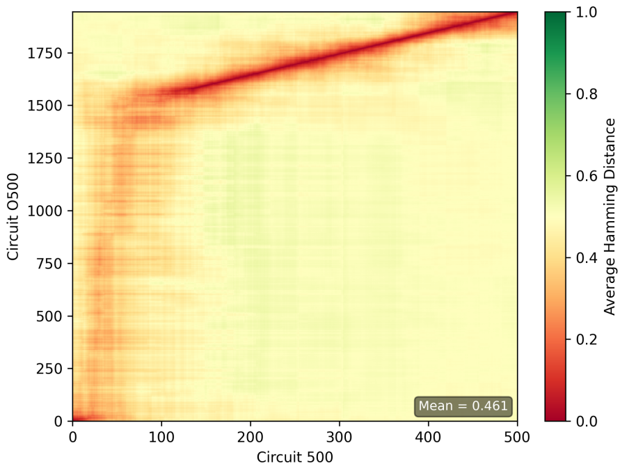
Figure 19: Heatmap showing circuit 500 during compression: 1900 gates.
