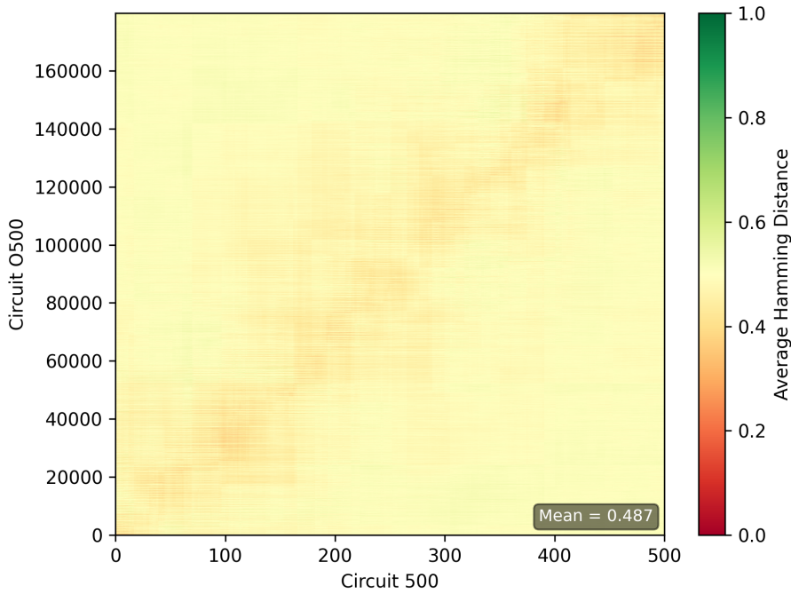
Figure 17: Heatmap showing circuit 500 before compression: 170,000 gates.
