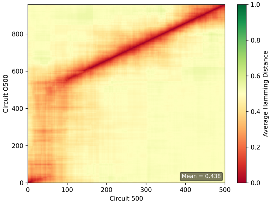
Figure 20: Heatmap showing circuit 500 after compression: 900 gates.
