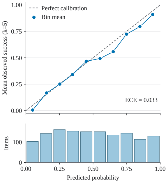
Calibration on 1,375 test questions
