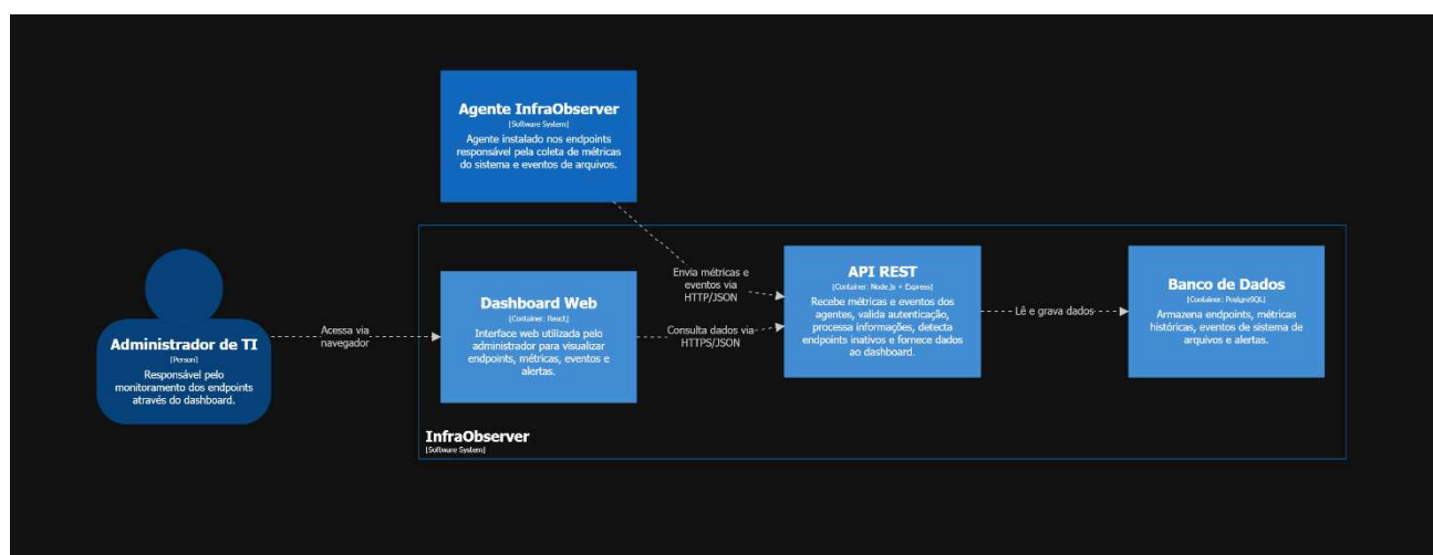
Figura 14: Diagrama de containers.
