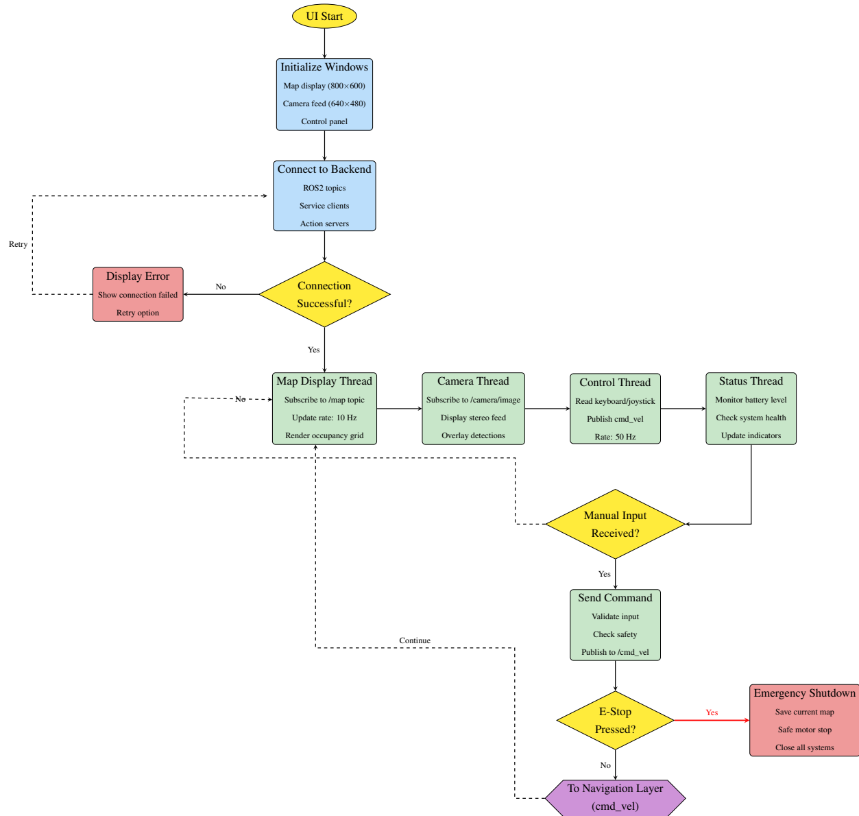
Figure 77: User Interface Layer Process Flow
