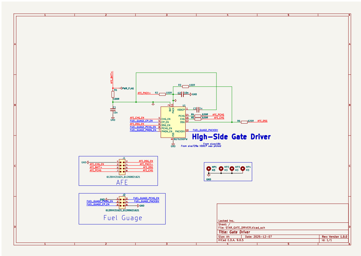
Figure 47: Gate Driver Schematic (BQ76200)
