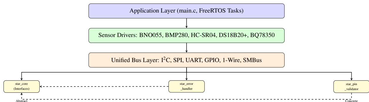
Figure 74: STAR Firmware Layered Architecture
