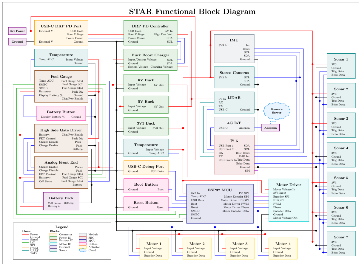
Figure 2: System Functional Block Diagram
