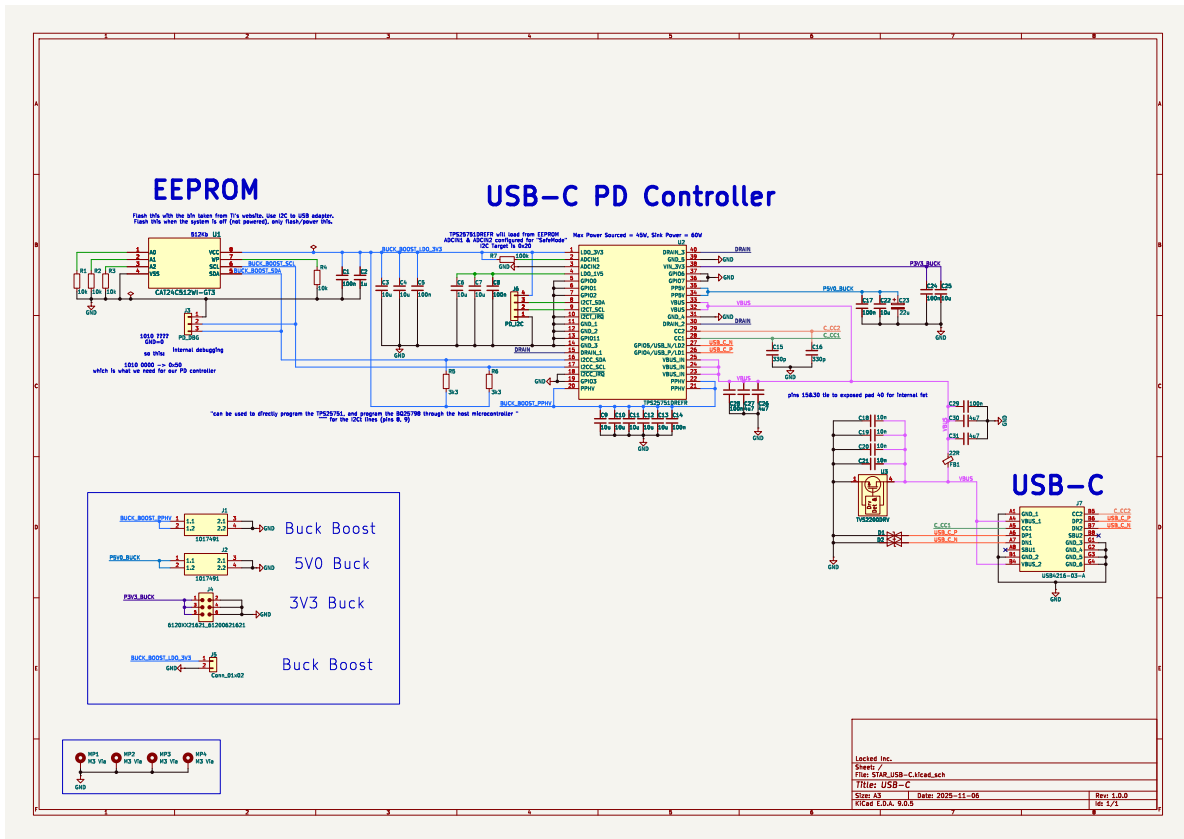
Figure 45: USB-C PD Controller Schematic (TPS25751D)
