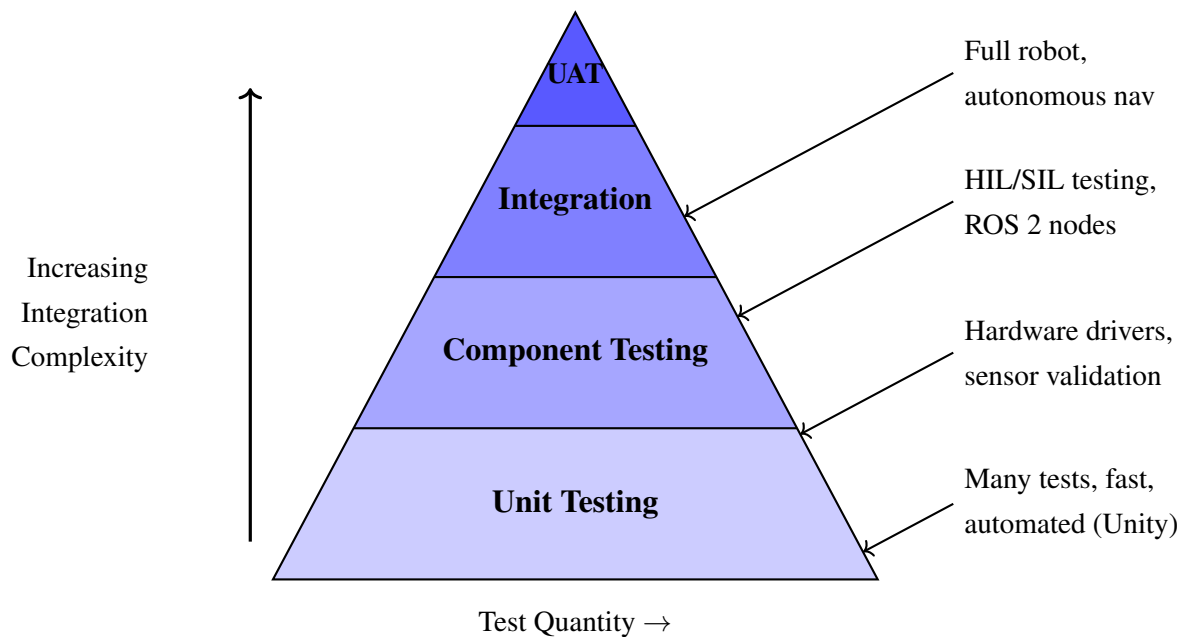
Figure 94: The Testing Pyramid showing the distribution of test types. Unit tests form the broad base with many fast, automated tests. Each successive level has fewer tests but validates increasingly complex integration. UAT = User Acceptance Testing.
