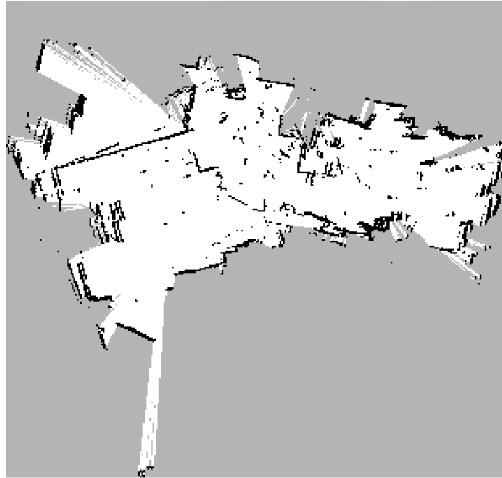
Figure 2: A finished SLAM occupancy grid produced by STAR in Thompson Hall on the Texas A&M campus. White cells are free space, black cells are detected obstacles (walls, doorways, furniture), and grey is unobserved. This is the same image format the Grafana cockpit map panel and the http://100.64.0.6:9101/map.png endpoint serve; download .pgm and .yaml from the cockpit (see Figure 3) to feed the map back into Nav2.
