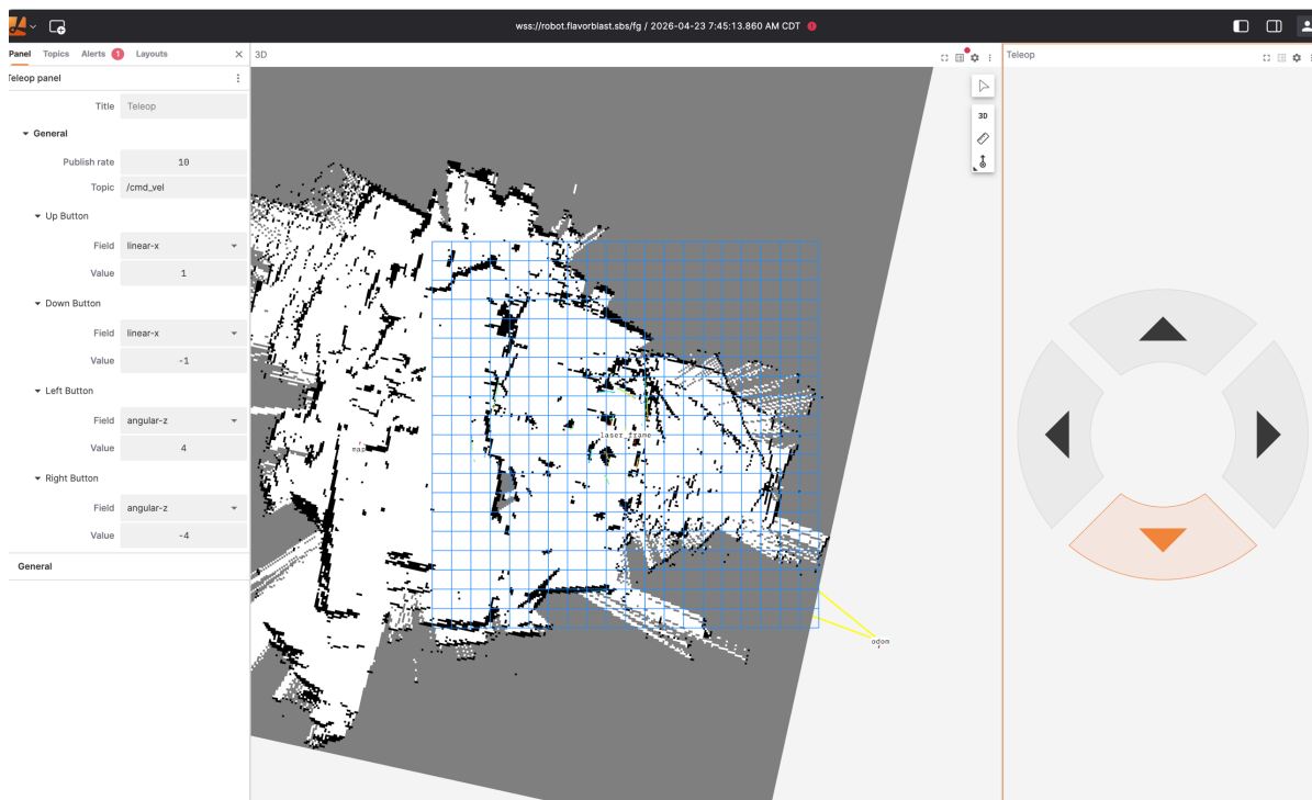
Figure 4: Lichtblick layout in operator use. The center 3D panel shows the live SLAM map (occupancy grid) with the laser_frame and odom TF axes overlaid. The right-rail Teleop panel publishes geometry_msgs/Twist on /cmd_vel at 10 Hz; the down-arrow is highlighted because it is being held. The left sidebar exposes the per-button linear-x / angular-z bindings the layout uses.
