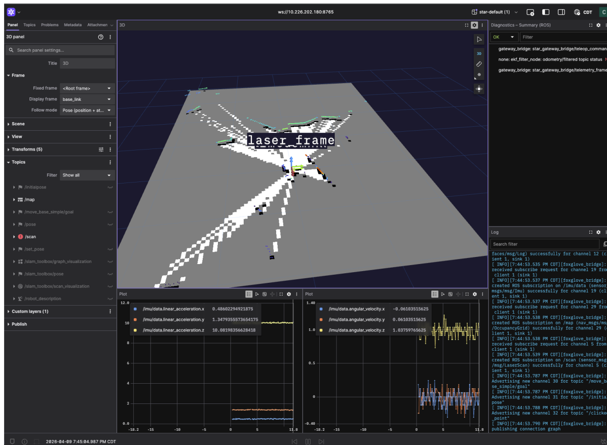
Figure 5: Foxglove Studio desktop app reading the same layout JSON the web Lichtblick uses. Center: live 3D scene with the /scan rays around laser_frame on top of the SLAM occupancy grid. Bottom: time-series plots of /imu/data.linear_acceleration and angular_velocity on all three axes. Right: the Diagnostics summary and the foxglove-bridge log stream.
