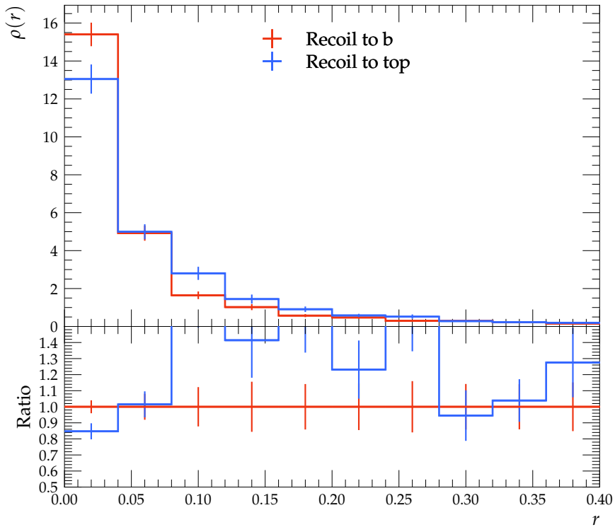
Differential jet shape for light-jets with 100 \text{ GeV} < p_T < 150 \text{ GeV}
