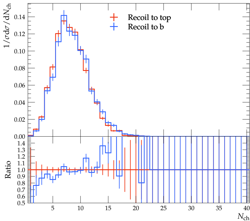
Charged particle multiplicity for B -jets 50 \text{ GeV} < p_T < 70 \text{ GeV}
