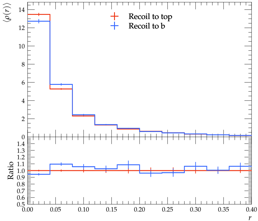
Differential jet shape B -jets 150 \text{ GeV} < p_T < 300 \text{ GeV}
