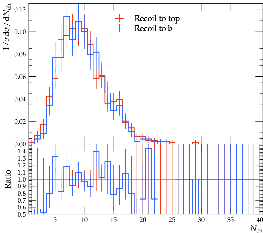
Charged particle multiplicity C-jets 100 \text{ GeV} < p_T < 150 \text{ GeV}
