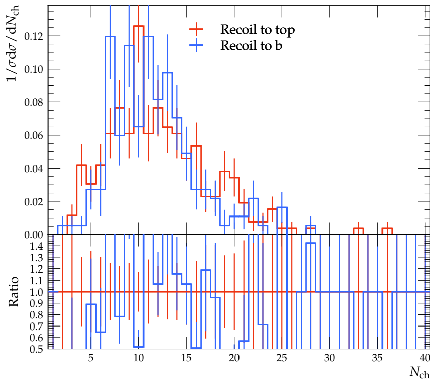
Charged particle multiplicity C-jets 150 \text{ GeV} < p_T < 300 \text{ GeV}
