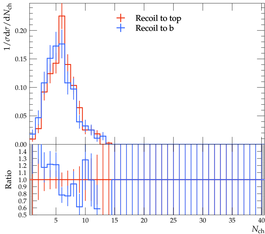
Charged particle multiplicity C-jets 25 \text{ GeV} < p_T < 30 \text{ GeV}
