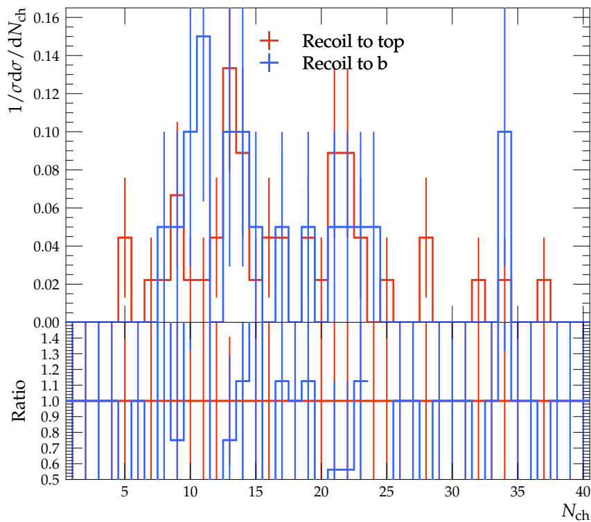
Charged particle multiplicity C-jets 300 \text{ GeV} < p_T < 500 \text{ GeV}
