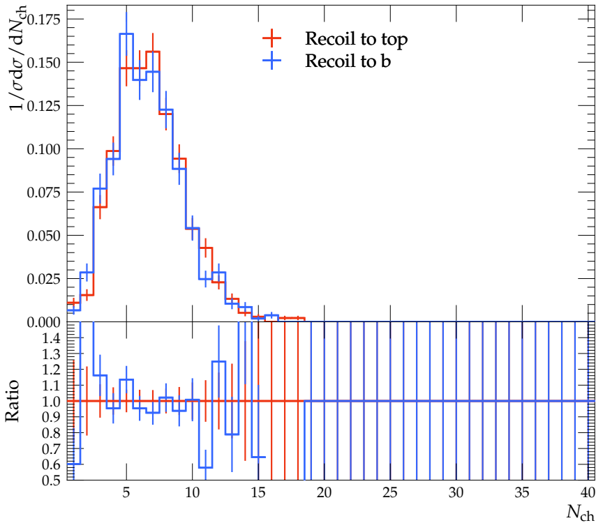
Charged particle multiplicity C-jets 30 \text{ GeV} < p_T < 50 \text{ GeV}
