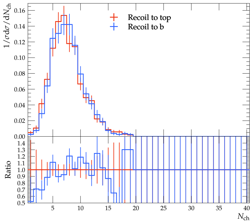
Charged particle multiplicity C-jets 50 \text{ GeV} < p_T < 70 \text{ GeV}
