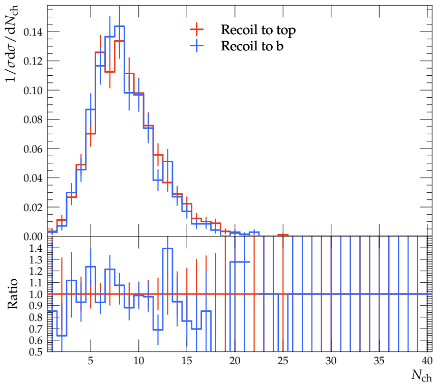
Charged particle multiplicity C-jets 70 \text{ GeV} < p_T < 100 \text{ GeV}
