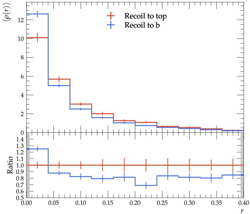
Differential jet shape C-jets 100 \text{ GeV} < p_T < 150 \text{ GeV}
