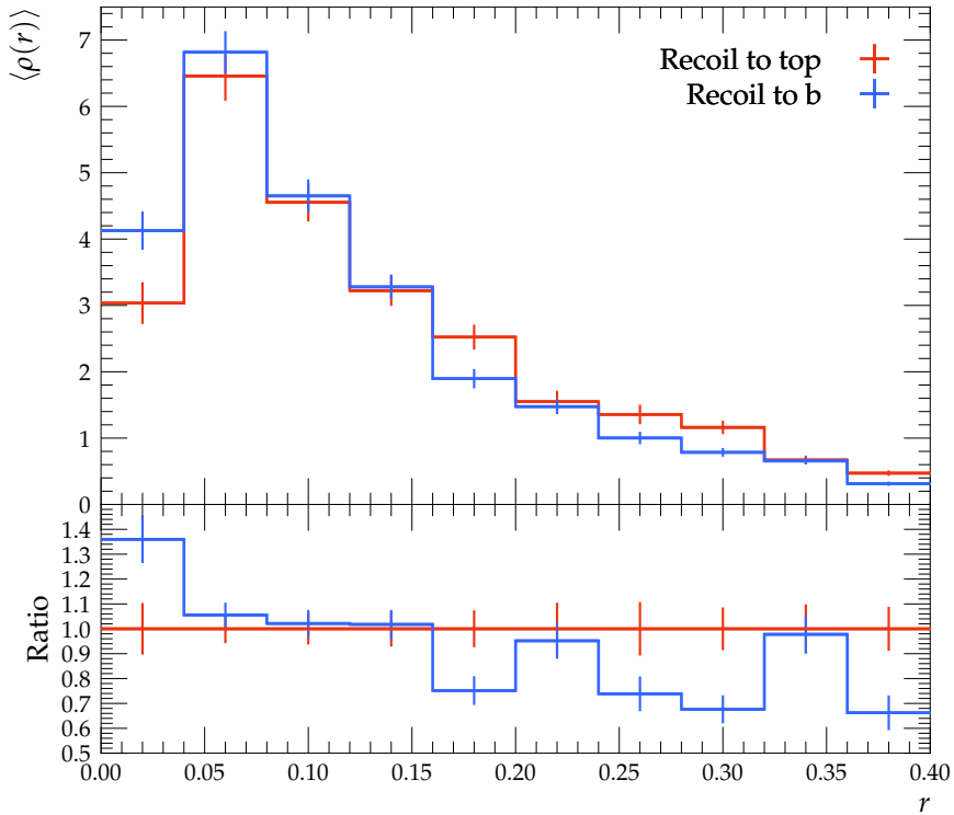
Differential jet shape C-jets 25 \text{ GeV} < p_T < 30 \text{ GeV}
