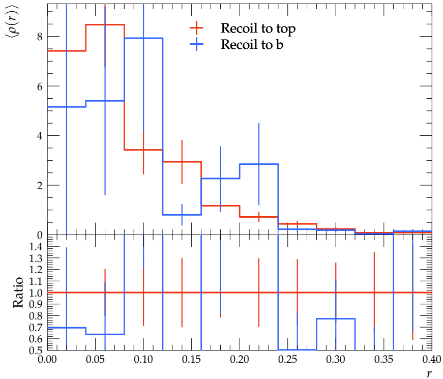
Differential jet shape C-jets 500 \text{ GeV} < p_T < 1000 \text{ GeV}
