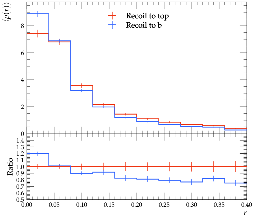
Differential jet shape C-jets 50 \text{ GeV} < p_T < 70 \text{ GeV}
