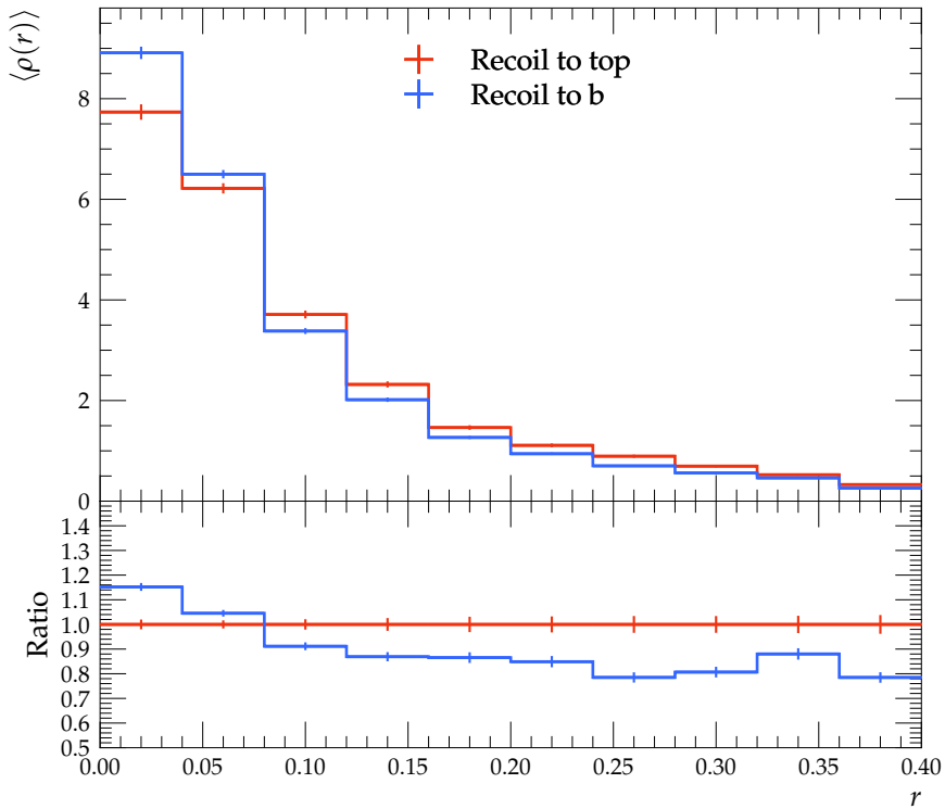
Differential jet shape for C-jets
