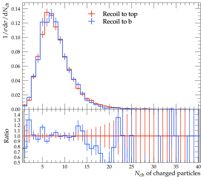
N_{\text{ch}} of charged, stable particles for C-jets
