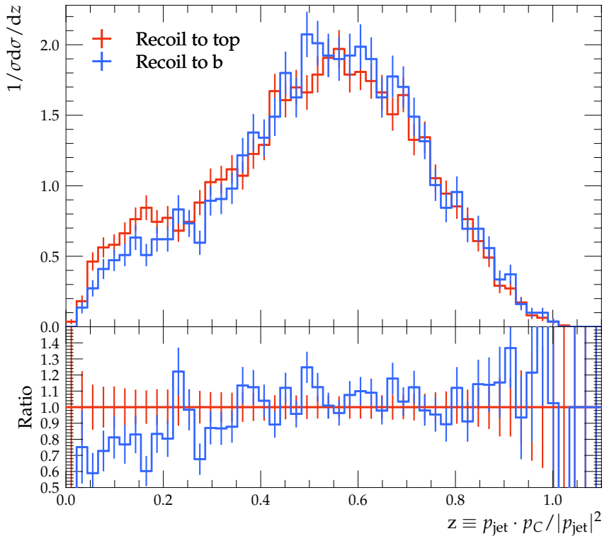
Fragmentation function for C-jets
