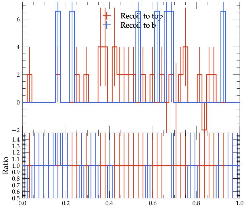
Fragmentation function for B -jets with 500 \text{ GeV} < p_{T,\text{jet}} < 1000 \text{ GeV}
