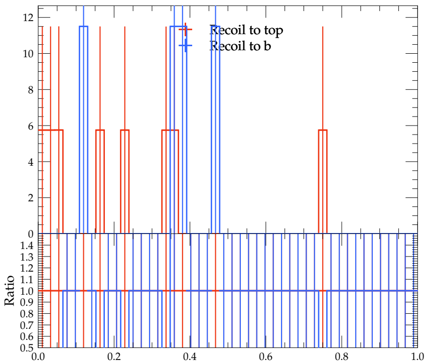
Fragmentation function for C-jets with exactly 1 HF hadron and 500 GeV <
