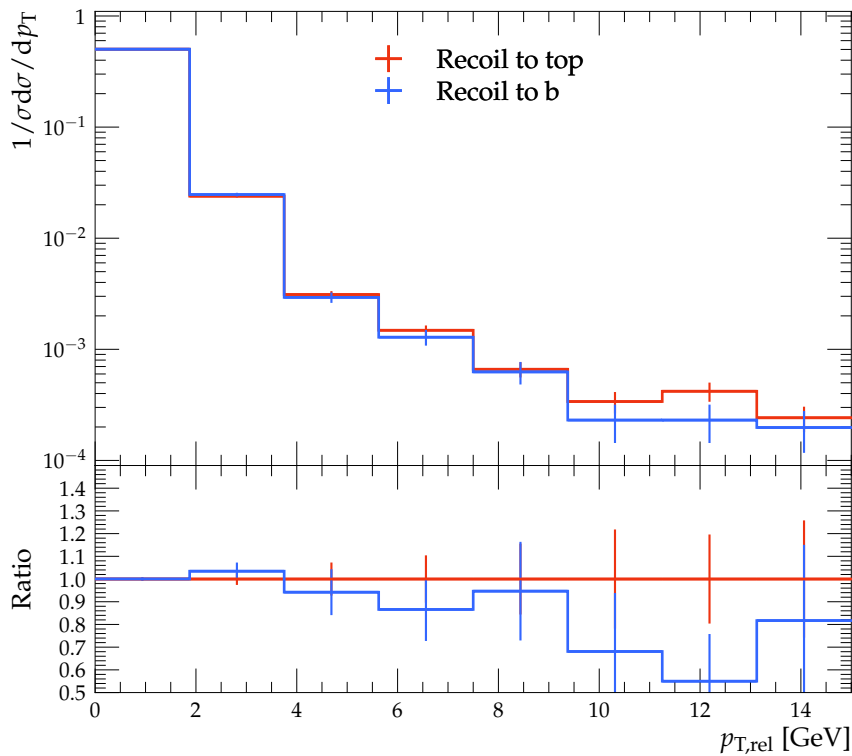
p_{T,\text{rel}} distribution for leptons in B -jets
