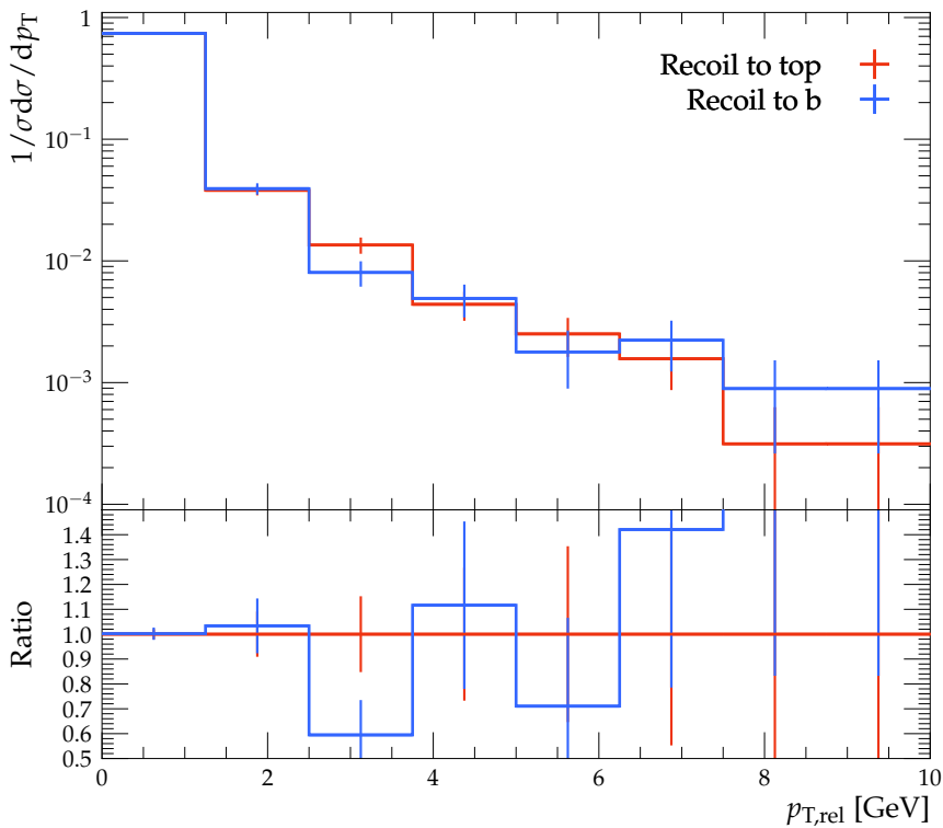
p_{T,\text{rel}} distribution for leptons in C-jets
