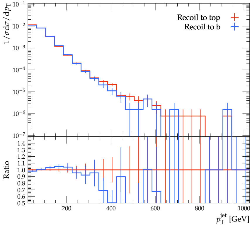
p_T^{\text{jet}} distribution for B -jets
