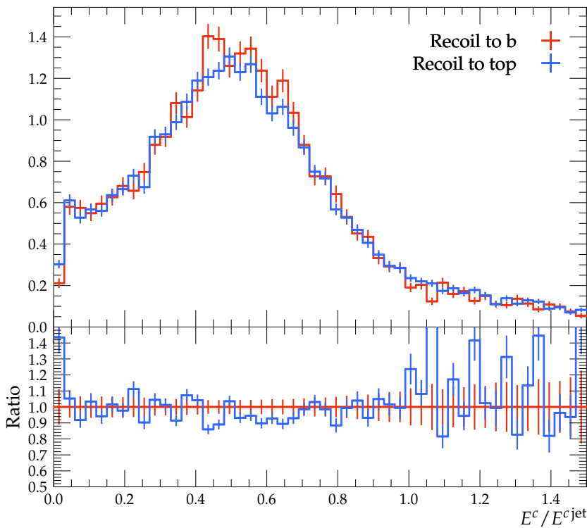
Energy fraction of c hadron in leading c jet
