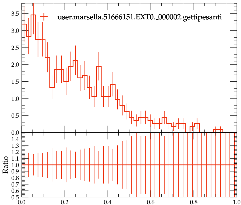
Fragmentation function for C-jets with 500 \text{ GeV} < p_{T,\text{jet}} < 1000 \text{ GeV}
