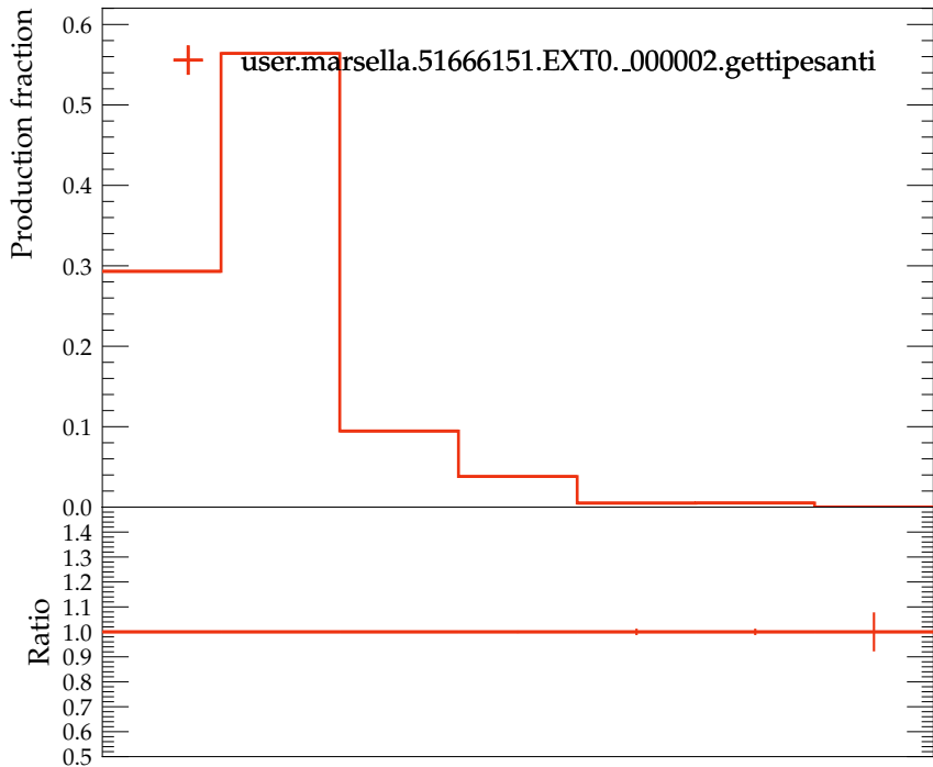
Production fractions for various weakly decaying c-hadrons
