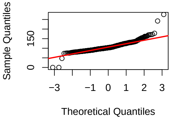
Normal Q-Q plot of runtime
