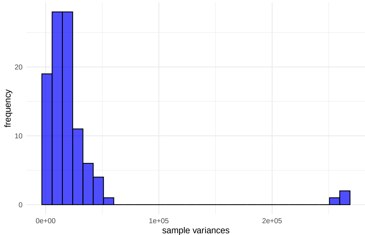
title = Distribution of variances sample
