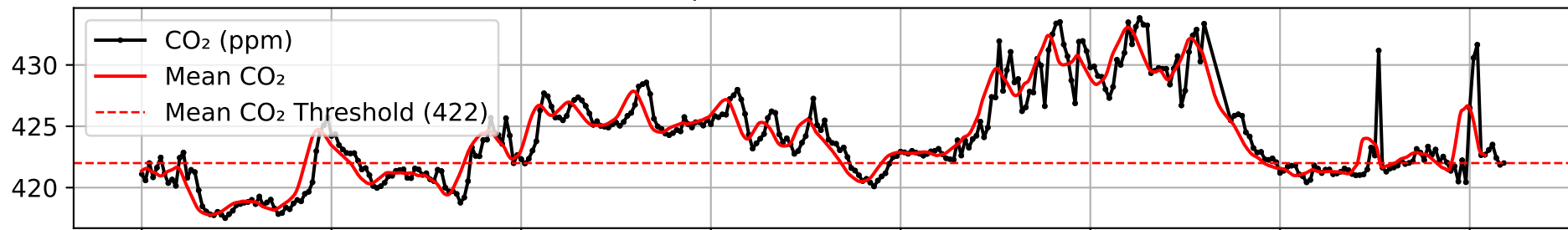
Atmospheric CO 2 Observations
