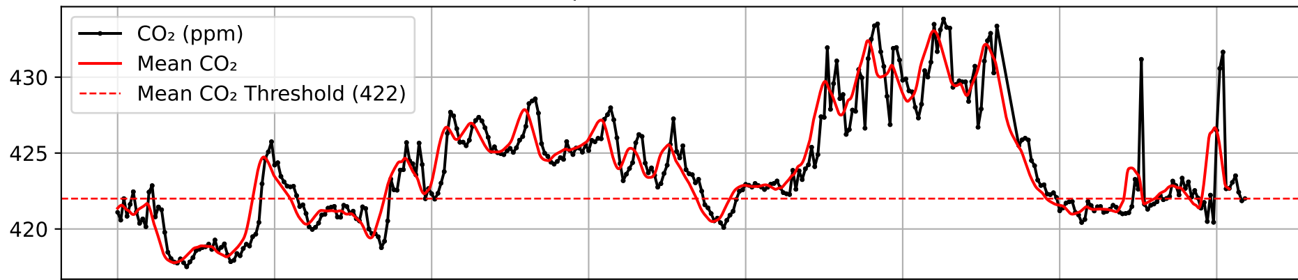
Atmospheric CO 2 Observations
