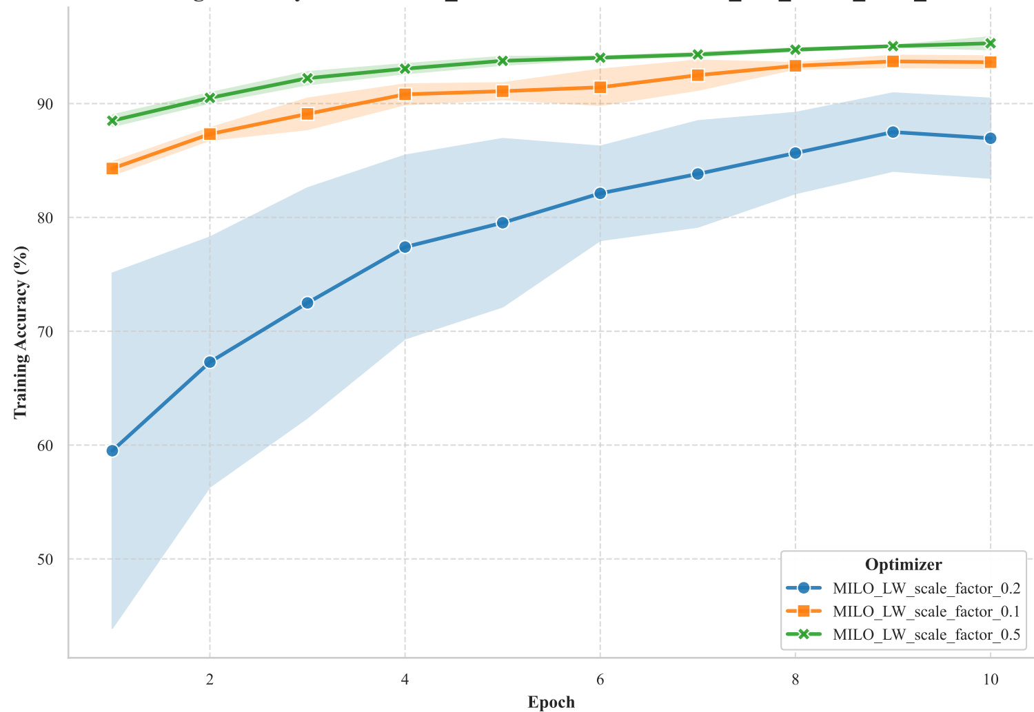
Training Accuracy for ResNet18_CIFAR10 Ablation: MILO_LW_ablate_scale_factor
