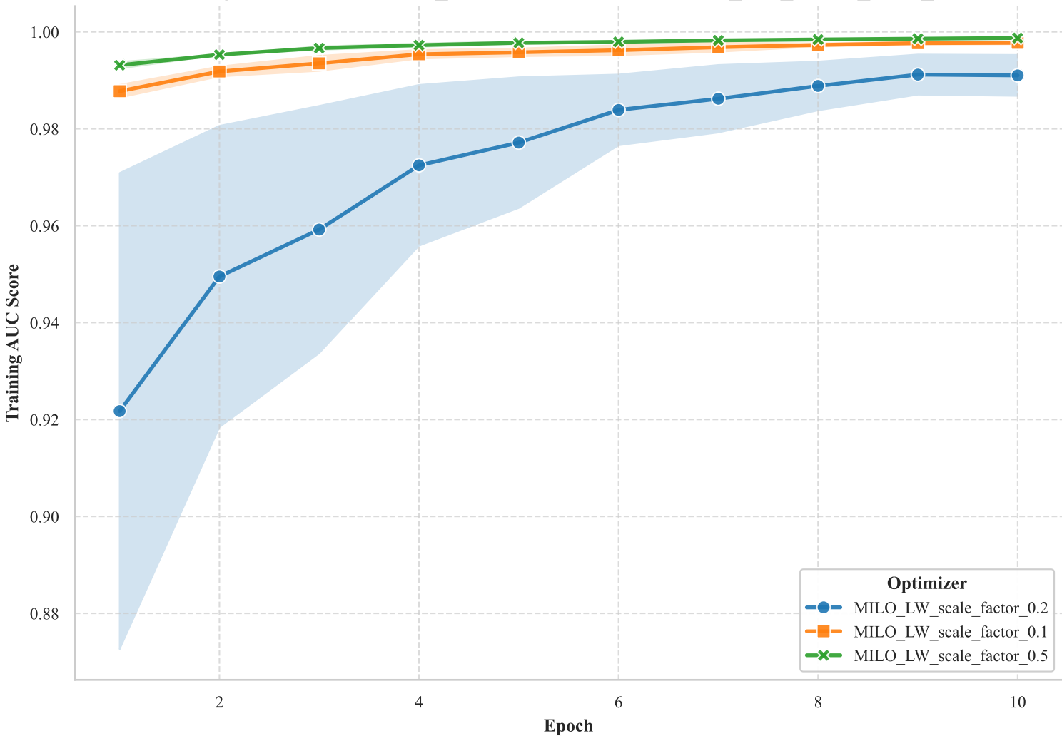
Training AUC for ResNet18_CIFAR10 Ablation: MILO_LW_ablate_scale_factor
