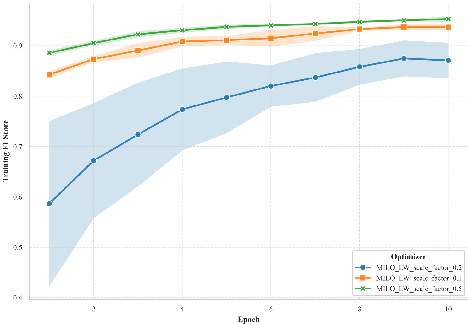
Training F1 Score for ResNet18_CIFAR10 Ablation: MILO_LW_ablate_scale_factor
