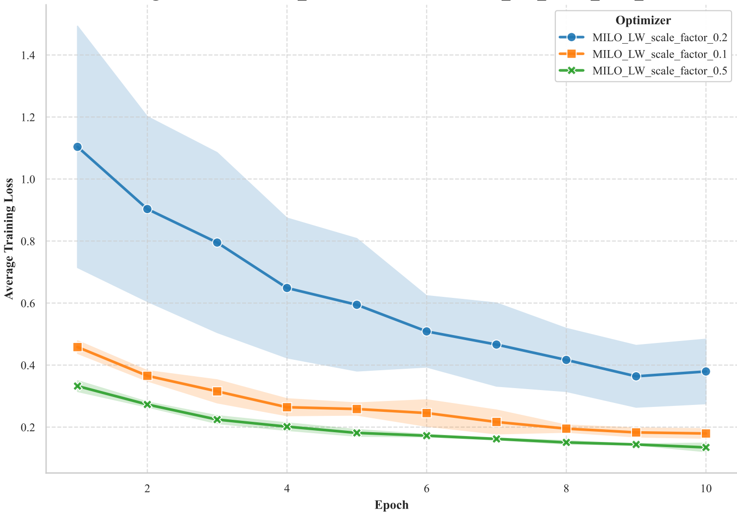
Training Loss for ResNet18_CIFAR10 Ablation: MILO_LW_ablate_scale_factor
