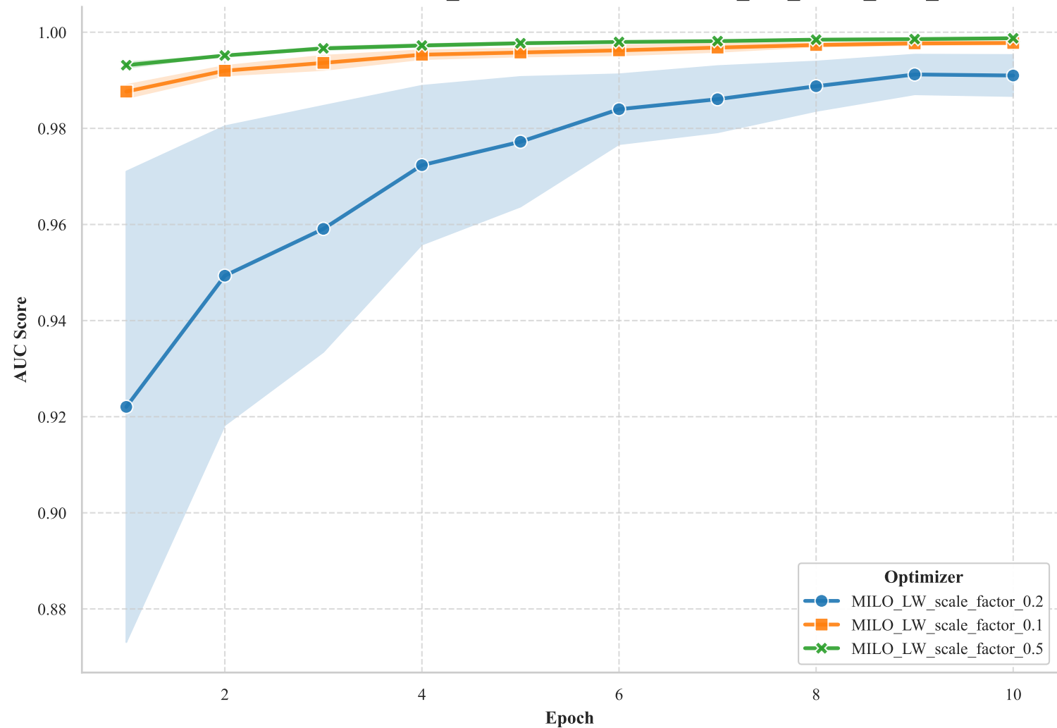
Validation AUC for ResNet18_CIFAR10 Ablation: MILO_LW_ablate_scale_factor
