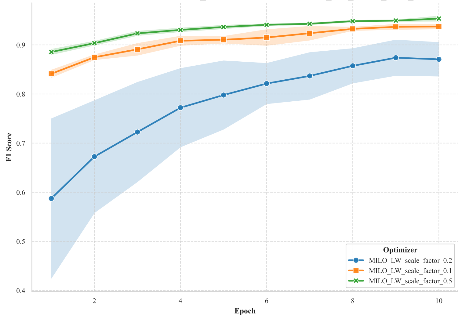
Validation F1 Score for ResNet18_CIFAR10 Ablation: MILO_LW_ablate_scale_factor
