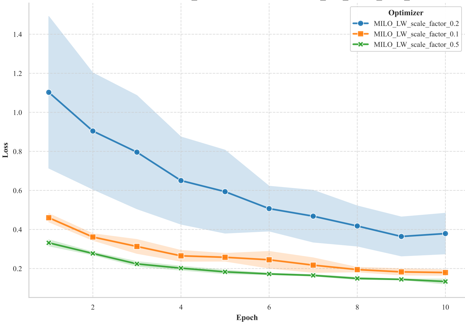
Validation Loss for ResNet18_CIFAR10 Ablation: MILO_LW_ablate_scale_factor
