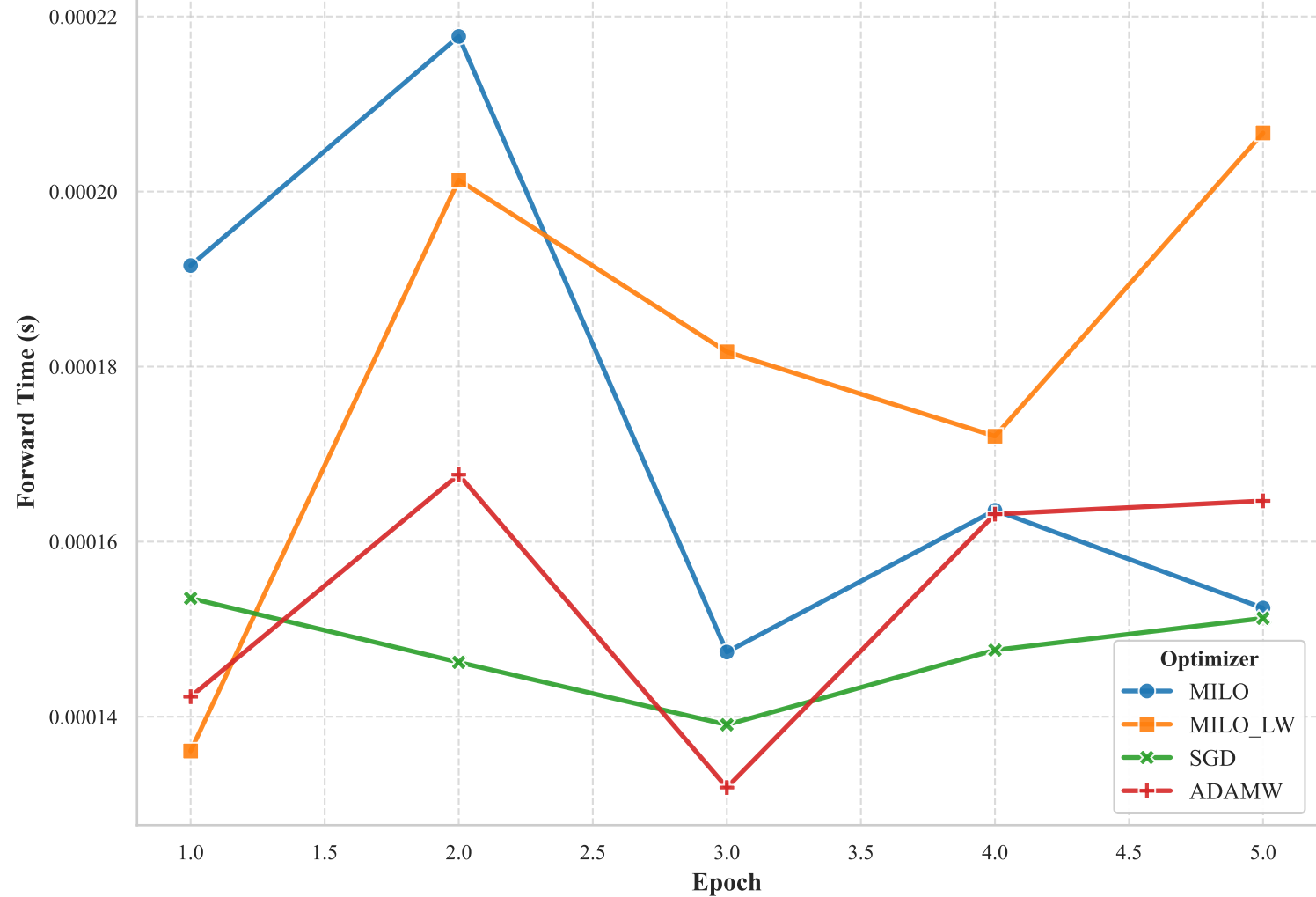
Forward Runtime per Epoch for LOGISTIC Experiment
