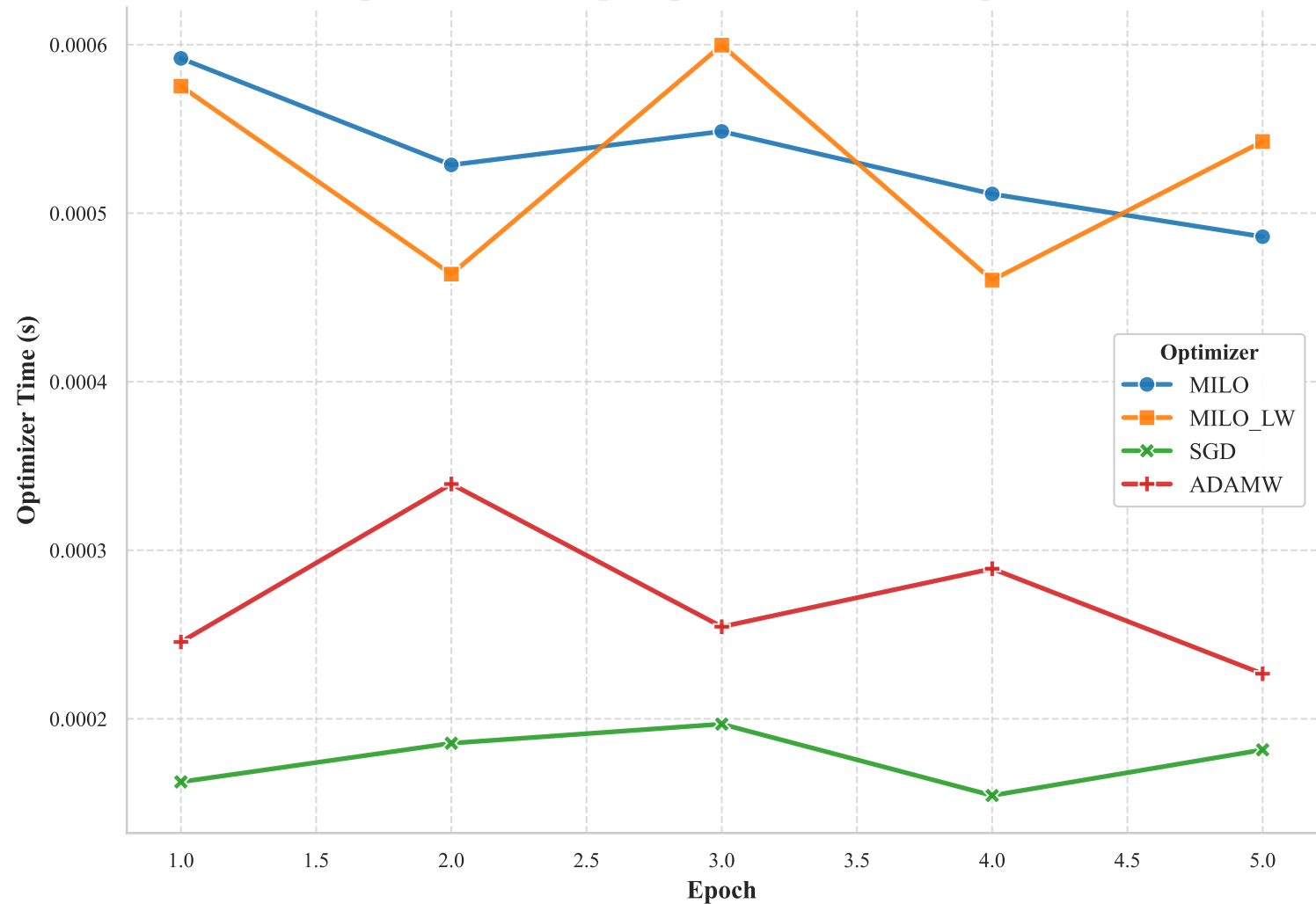
Optimizer Runtime per Epoch for LOGISTIC Experiment
