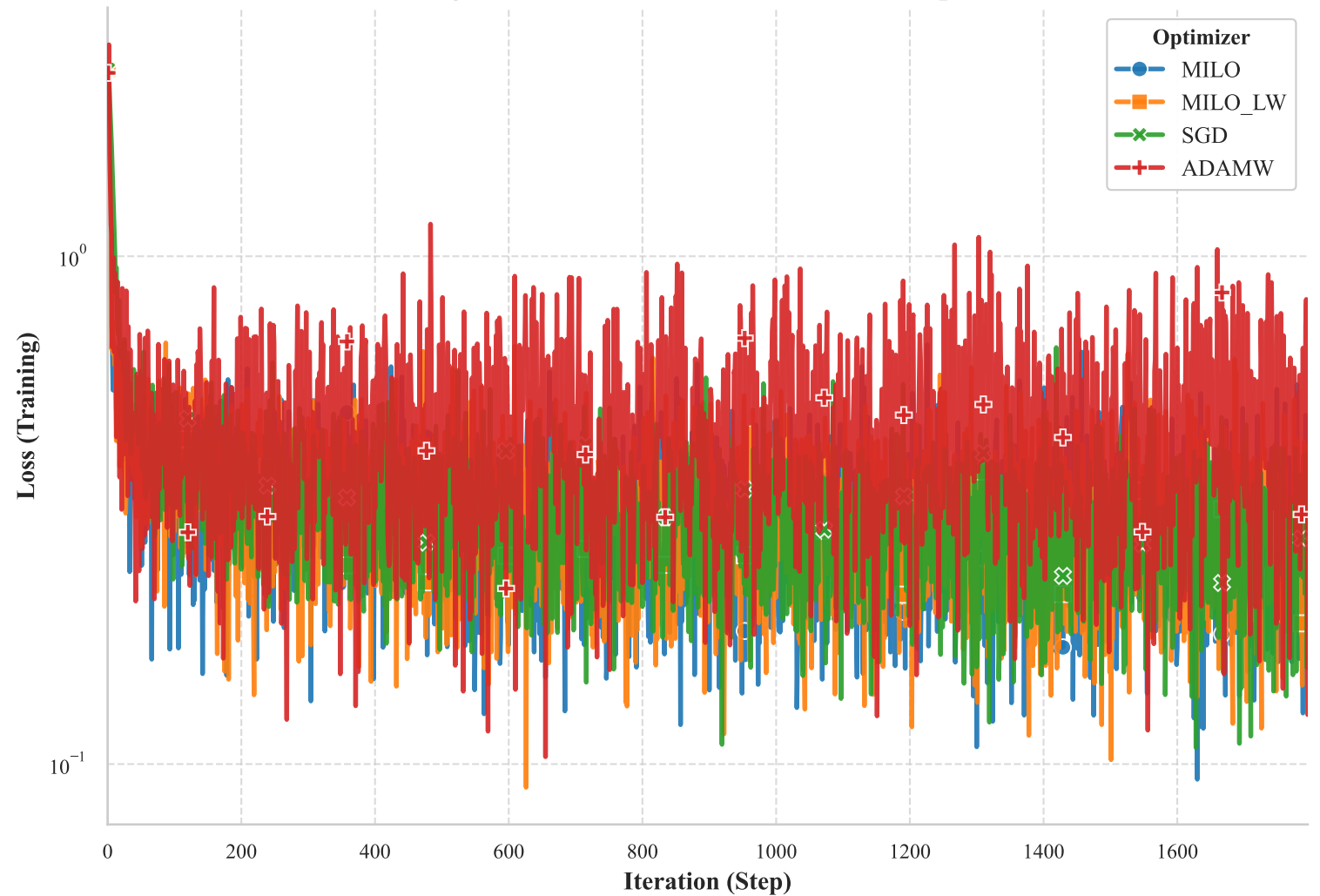
Training Loss vs. Iteration for LOGISTIC Experiment
