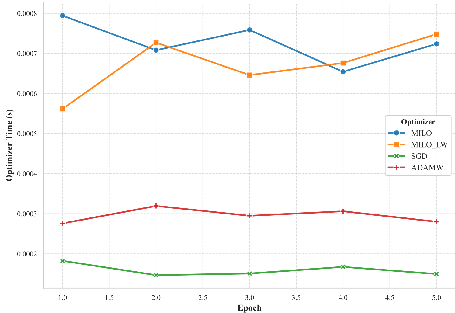
Optimizer Runtime per Epoch for MULTILAYER Experiment
