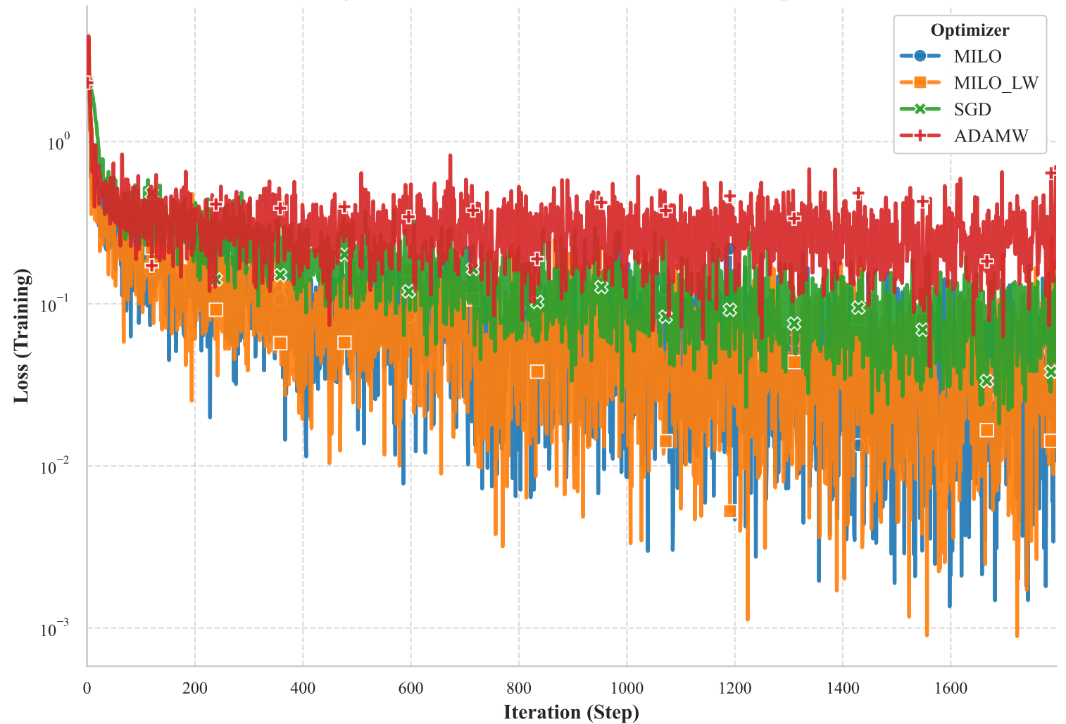
Training Loss vs. Iteration for MULTILAYER Experiment
