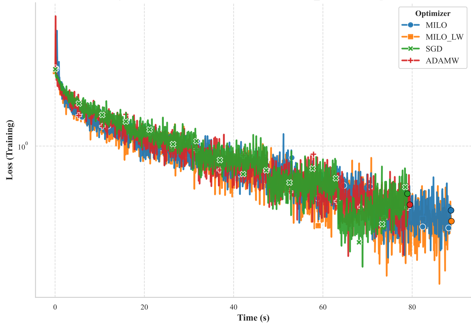
Training Loss vs. Wall-clock Time for RESNET34_CIFAR10 Experiment
