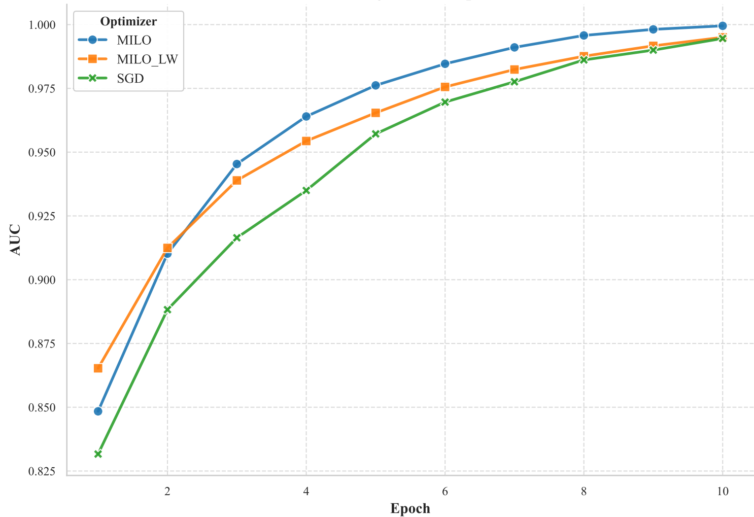
Training AUC vs. Epoch
