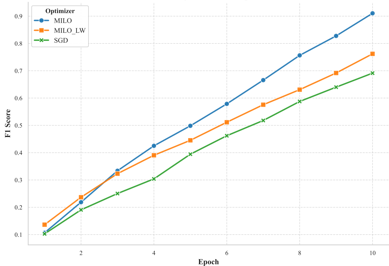
Training F1 Score vs. Epoch
