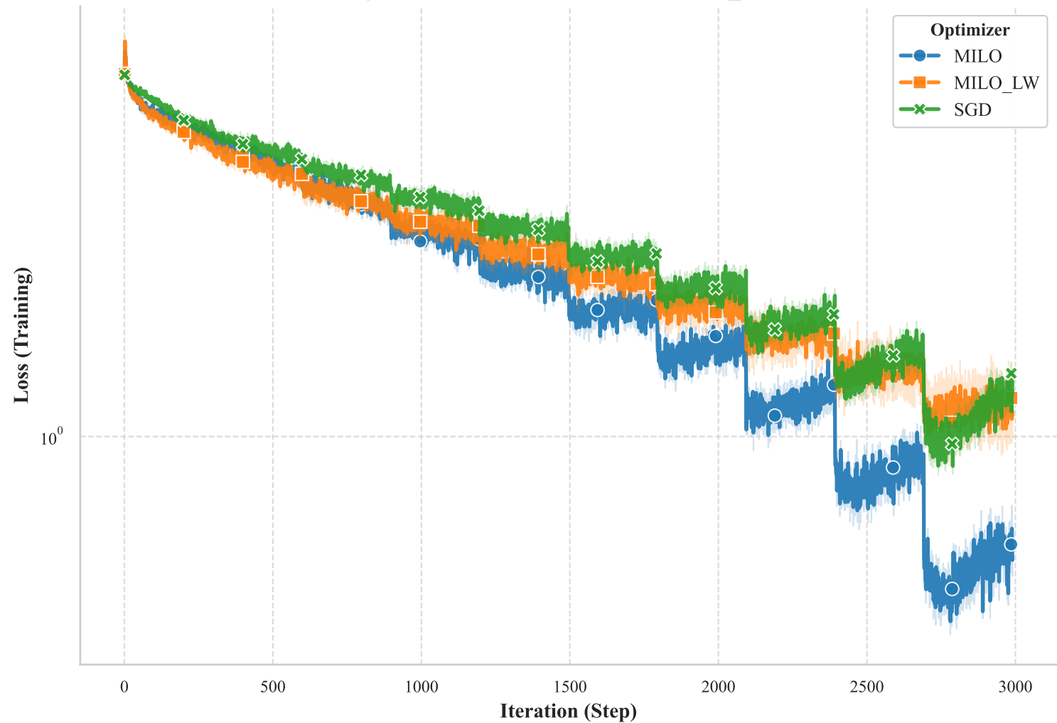
Training Loss vs. Iteration for RESNET34_CIFAR100
